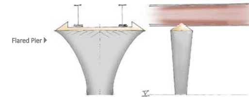
▲ Pier geometry varies dramatically based on dual girder and truss superstructure types.
