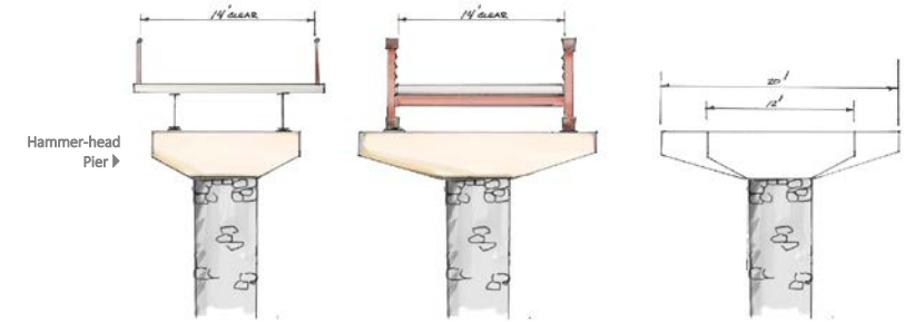
▲ Pier geometry varies dramatically based on dual girder and truss superstructure types.
